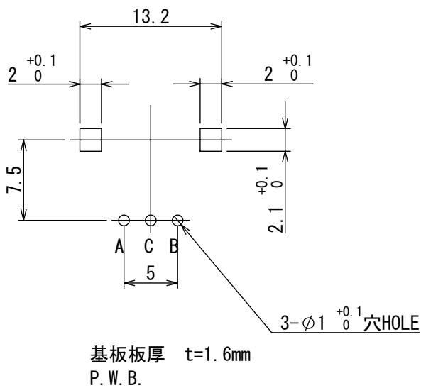
取付穴寸法図 (許容差±0.1) * 挿入側より見た図 P.W.B. MOUNTING DETAIL (TOLERANCE±0.1) VIEWED FROM MOUNTING SIDE
