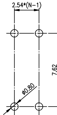
RECOMMENDED P.C.B. LAYOUT (TOP VIEW)
