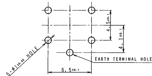
P.C BOARD MOUNTING HOLE DIMENSIONS (WHEN VIEWED FROM SWITCH MOUNTING FACE)
