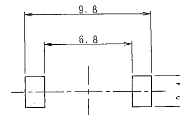
推奨ハ°ターン図 (5:1) PRINTED CIRCUIT BOARD MOUNTING LAND DIMENSION (WHEN VIEWED FROM SWITCH MOUNTING FACE)
