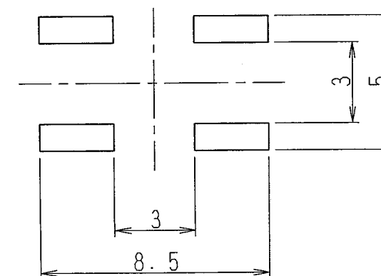
PRINTED CIRCUIT MOUNTING HOLE DIMENSION 推奨パターンの図 (WHEN VIEWED FROM SWITCH MOUNTING FACE) (スイッチ取り付け面より見る)
