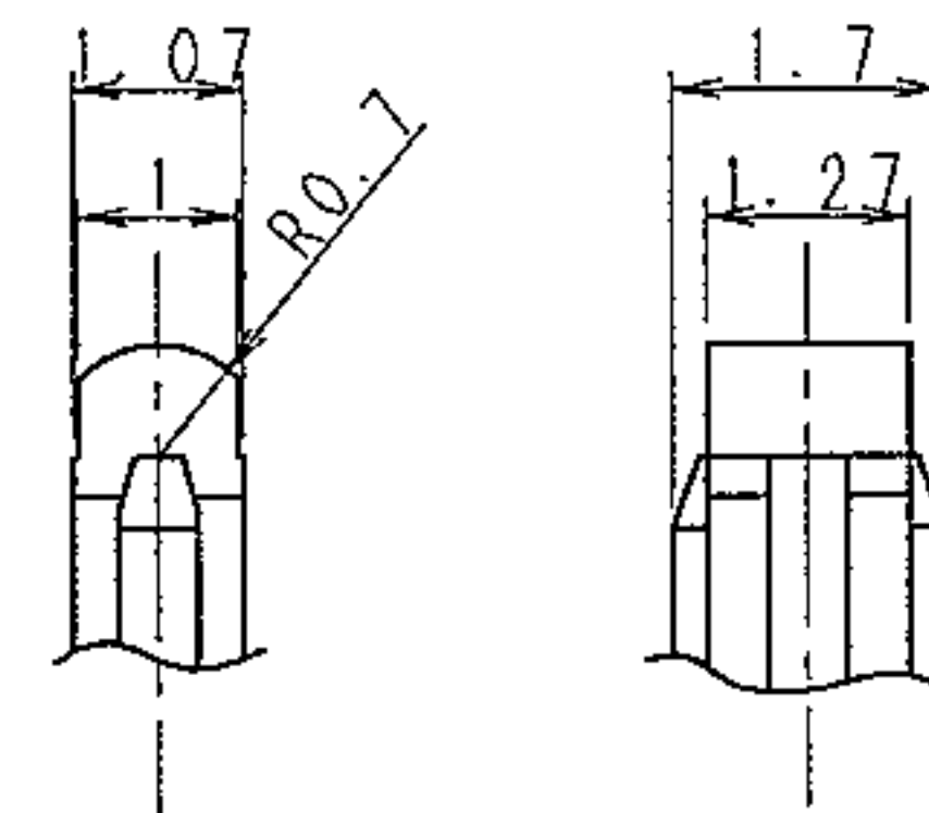
REFERENCE DRAWING FOR MOUNTING HOLES (5:1)
