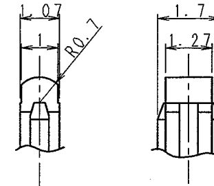
REFERENCE DRAWING FOR MOUNTING HOLES (5:1)
