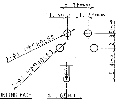
REFERENCE DRAWING FOR MOUNTING HOLES (5:1)
