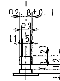
②DETAIL (詳細) (2/1)
