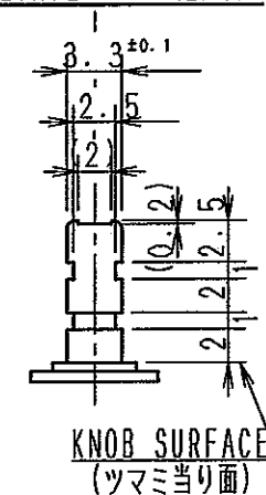
①DETAIL (詳細) (2/1)
