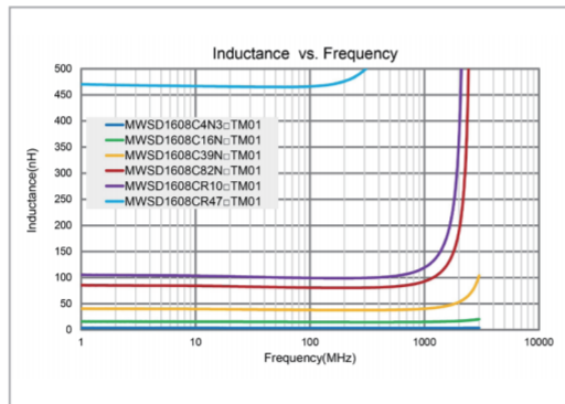
MWSD1608C-M01 TYPE Inductance vs. Frequency Characteristics
