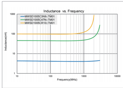
MWSD1005C-M TYPE Inductance vs. Frequency Characteristics
