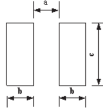
Recommended Land Pattern
