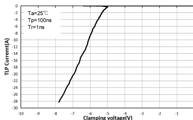
TLP IV curve Pin2 to Pin1
