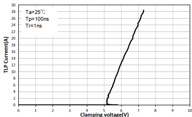
TLP IV curve Pin1 to Pin2
