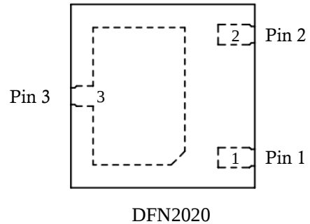
DFN2020
