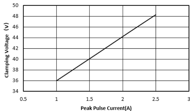
Clamping Voltage VS Peak Pulse Current( t_p=8/20\mu\text{s} )
