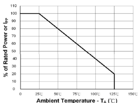
Figure 1. Power Detating
