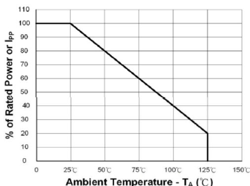
Figure 1. Power Detating
