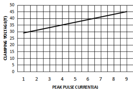
Figure 2. Clamping Voltage vs. I_{PP}
